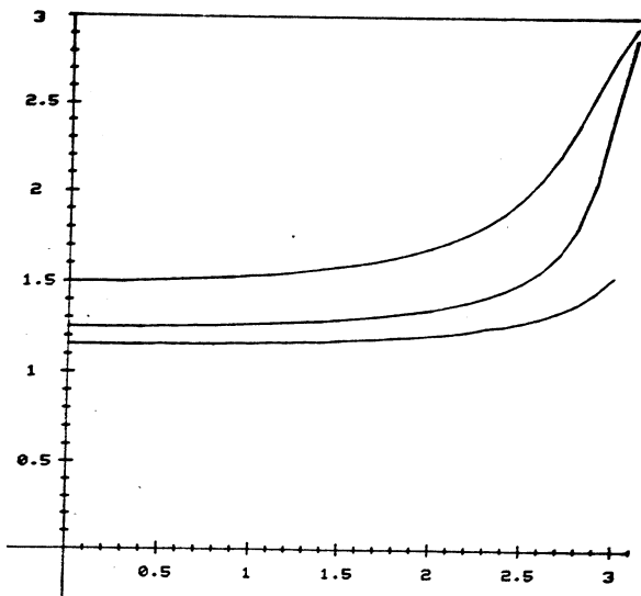
Fig. 11. Mass ratios for simple terminating orbits. The values in Table II are presented graphically. The vertical axis gives the mass ratio ( \mu ); the horizontal axis is the starting angle ( \theta_0 ) in radians. The top line, at \mu = 3 , is for type B1; the next graph down is type B2; next comes type B3; and the bottom graph is type B4.
