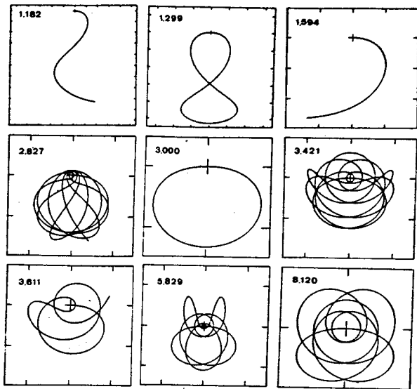
Fig. 6. Terminating trajectories. Mass ratio ( \mu ) in upper left corner. Swinging mass again launched from the center, with \theta_0 = 90^\circ and \dot{r}_0 = 4 .
