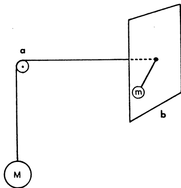
Fig. 2. Laboratory model of SAM. (a) Air pulley. (b) Air table, mounted vertically.
