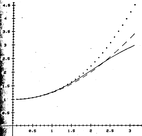
Fig. 8. Mass ratios for type A. The values in Table I are graphed. The vertical axis represents the mass ratio ( \mu ); the horizontal axis is starting angle ( \theta_0 ), in radians. The solid line gives the computer results; the dashed line gives the theoretical estimate of Eq. (15); the dotted line is the theoretical estimate of Eq. (17).
