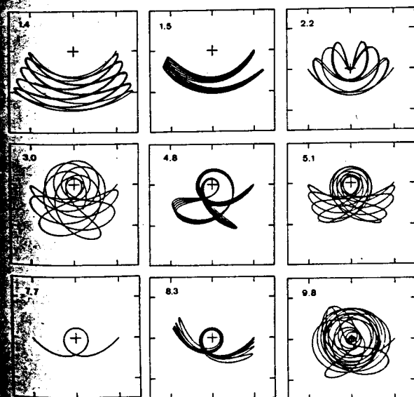
Fig. 3. Nonsingular trajectories. The mass ratio ( \mu ) is given in the upper corner of each graph. The center ( r = 0 ) is indicated with a cross. In each case the swinging bob was released from rest one unit to the right of center.
