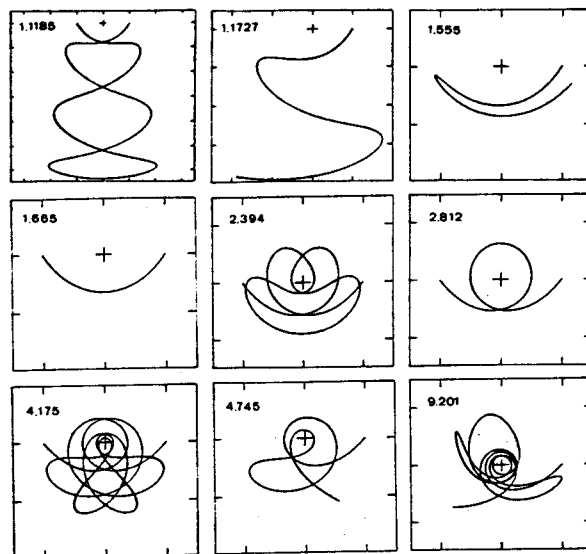
Fig. 4. Periodic trajectories. Mass ratio ( \mu ) is given in the upper left corner of each graph. Swinging mass again released from rest at r_0 = 1 , \theta_0 = 90^\circ .
